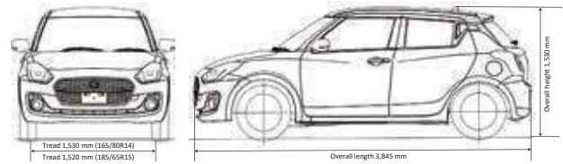
The drawings shown are general specifications of the vehicle.
